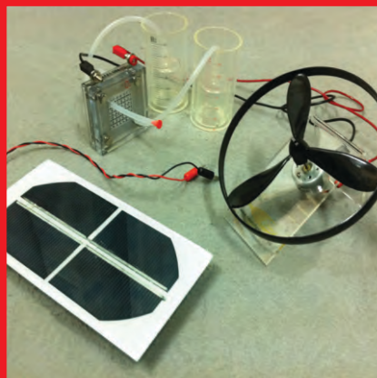
Solar energy kit
